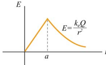
Figure 4.2.16 Electric field due to a uniformly charged sphere as a function of r .
