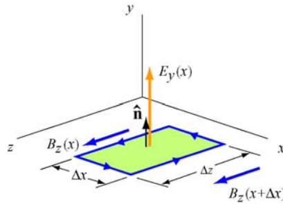
Figure 13.4.3 Spatial variation of the magnetic field \vec{B}
