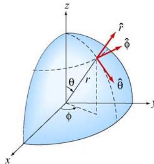
Figure 1.2.3 Spherical coordinates
