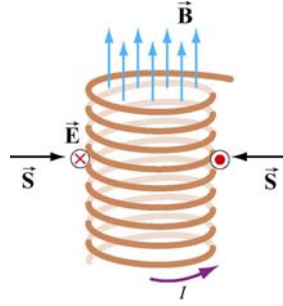
Figure 13.6.4 Poynting vector for a solenoid with dI / dt > 0
