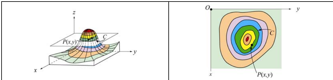
Figure 3.5.4 A topographic map
