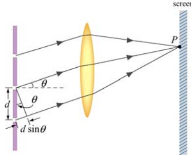
Figure 14.8.1 Diffraction grating
