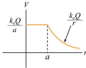
Figure 4.3.7 Electric potential as a function of r for a spherical conducting shell
