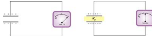
Figure 5.5.5 Inserting a dielectric material between the capacitor plates while keeping the charge Q_0 constant
