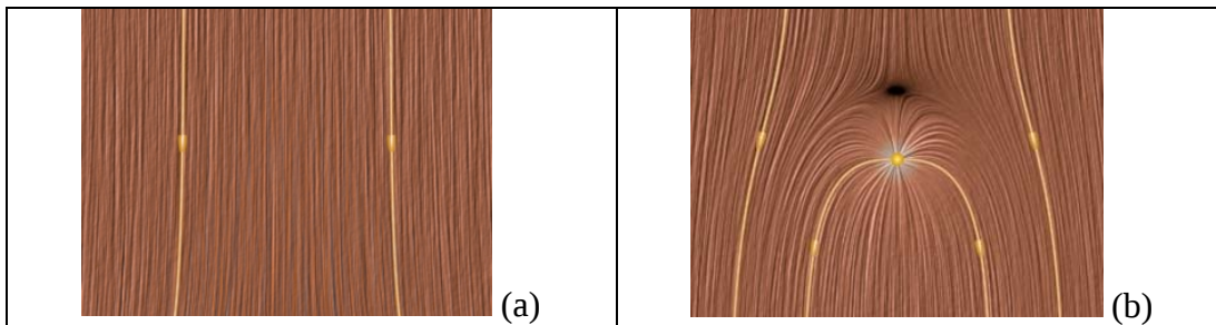
Figure 4.6.2 A positive charge moving in a constant electric field which points downward. (a) The total field configuration when the charge is still out of sight on the negative z -axis. (b) The total field configuration when the charge comes to rest at the origin, before it moves back down the negative z -axis.
