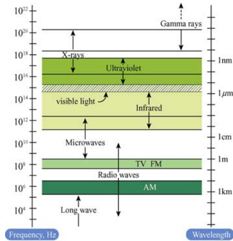
Figure 13.4.4 Electromagnetic spectrum
